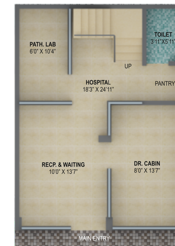
GROUND FLOOR PLAN AREA - 760 SQ. FT.
