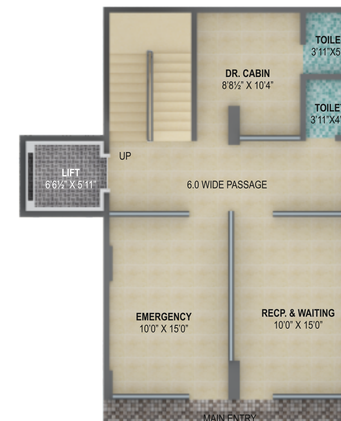
GROUND FLOOR PLAN AREA - 1115 SQ. FT.
