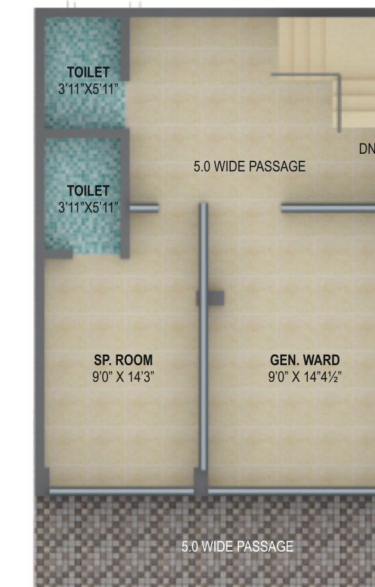
SECOND FLOOR PLAN AREA - 765 SQ. FT.
