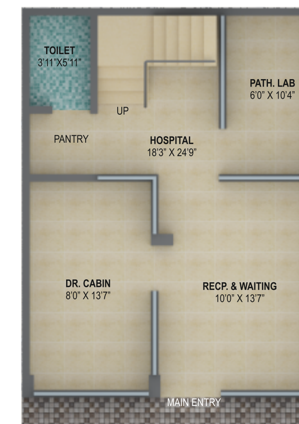
GROUND FLOOR PLAN AREA - 1000 SQ. FT.
