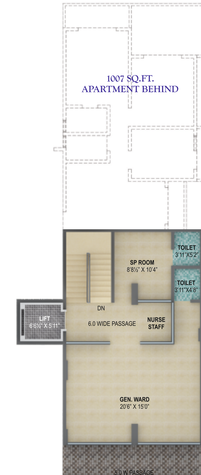
SECOND FLOOR PLAN AREA - 1115 SQ. FT.
