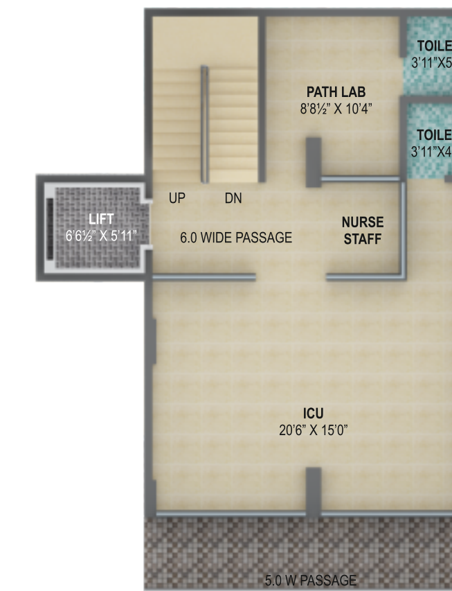
FIRST FLOOR PLAN AREA - 1115 SQ. FT.
