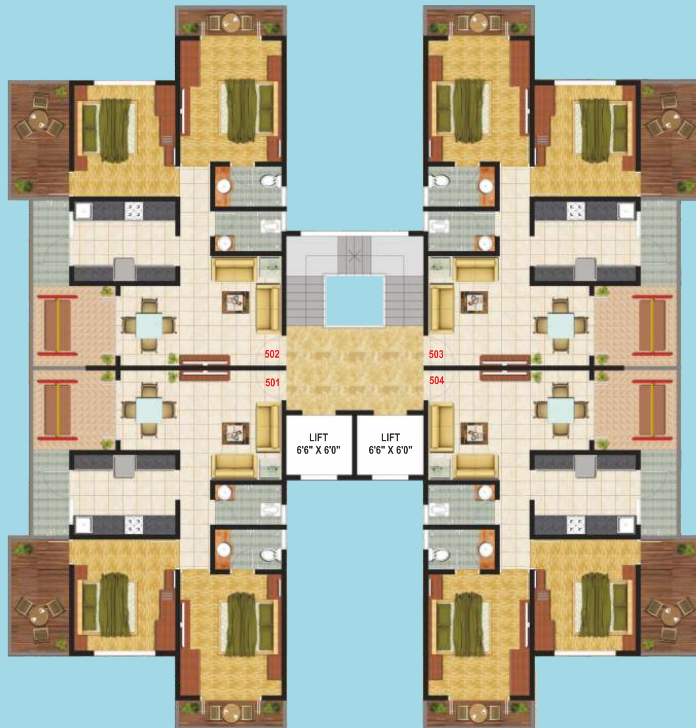
FLOOR PLAN : FIFTH FLOOR
